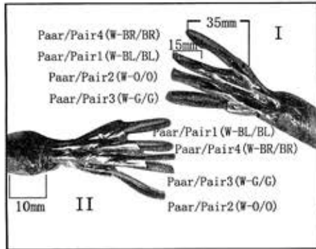
SF/UTP-S/STP
